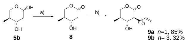
Scheme 2. Stereoselective alkylation. a) Br 2 , BaCO 3 , 12 h, 62%; b) LDA, HMPA, –78 °C, alkene bromide, 36 h. LDA = lithium diisopropylamide, HMPA = hexamethylphosphoramide.
