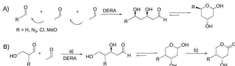
Scheme 1. Preparation of unnatural pyranoses with DERA. a) pH 7.5, DERA, acetaldehyde; b) Br 2 , BaCO 3 . For details of routes A and B see text.
